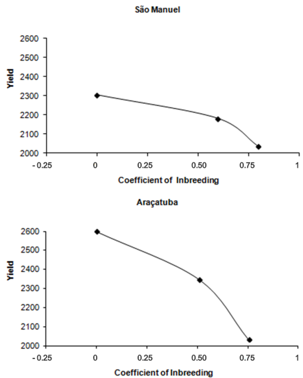
Figure 2. Coefficient of inbreeding x grain yield (kg ha -1 ) of Ricinus communis L. progenies in São Manuel and Araçatuba, SP.
