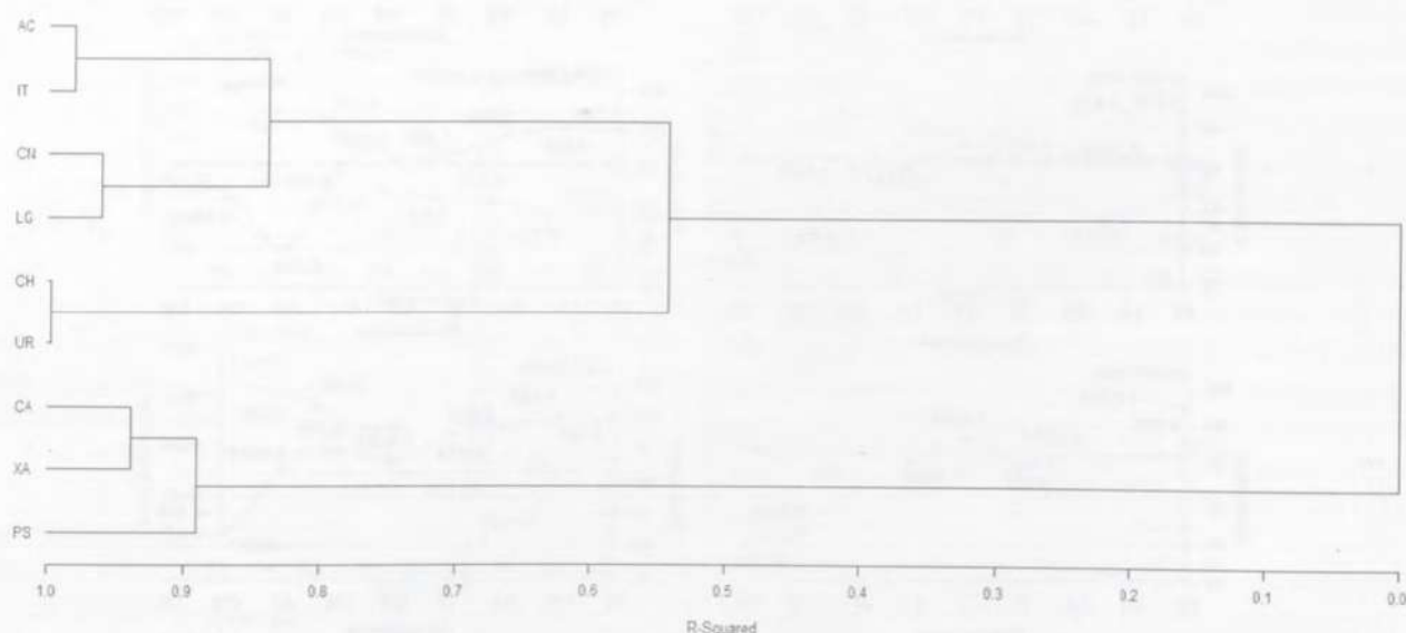
Figure 3. Dendrogram based on nine environments of the state of Santa Catarina ((Águas de Chapecó (AC), Campos Novos (CN), Canoinhas (CA), Chapecó (CH), Ituporanga (IT), Lages (LG), Ponte Serrada (PS), Urussanga (UR) and Xanxerê (XA)) for the traits grain yield and plant cycle in Carioca common bean genotypes
