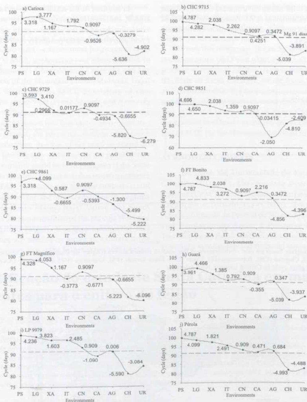
Figure 2. Values of the trait plant cycle and prediction of the environmental values by the BLUP method for 10 genotypes grown in nine environments ((Águas de Chapecó (AC), Campos Novos (CN), Canoinhas (CA), Chapecó (CH), Ituporanga (IT), Lages (LG), Ponte Serrada (PS), Urussanga (UR) and Xanxerê (XA)) of the state of Santa Catarina in the growing seasons of 2004/05, 2005/06 and 2006/07
