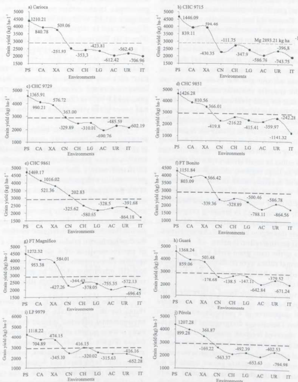
Figure 1. Values of the trait grain yield and prediction of the environmental values by the BLUP method for 10 genotypes grown in nine environments ((Águas de Chapecó (AC), Campos Novos (CN), Canoinhas (CA), Chapecó (CH), Ituporanga (IT), Lages (LG), Ponte Serrada (PS), Urussanga (UR) and Xanxerê (XA)) in the state of Santa Catarina in the growing season of 2004/05, 2005/06 and 2006/07
