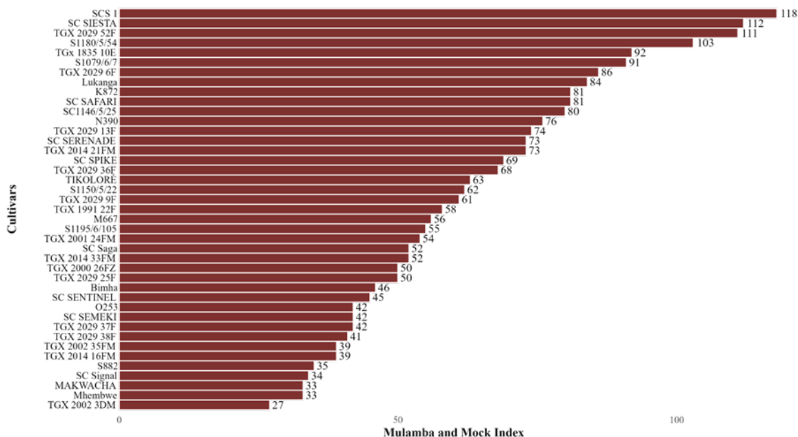
Figure 1. Ranking of soybean cultivars based on the Mulamba and Mock selection index for grain yield, biomass accumulation, and days to physiological maturity. Lower index values indicate superior overall performance across the evaluated traits.
